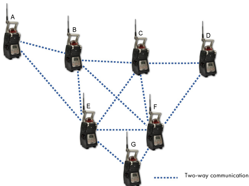
Figure 21 : In the example above, BM 25AW tag G communicates with E and F. In the event of a loss of communication between G and F, E still ensures the communication to the rest of the network. If G goes into gas alarm or fault condition, all BM 25AWs on the network will report a corresponding alarm
