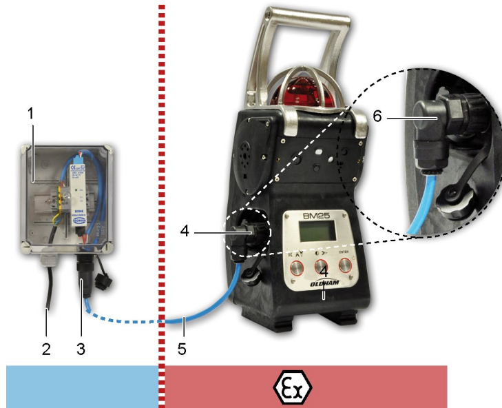
Figure 11: trickle charger connection
